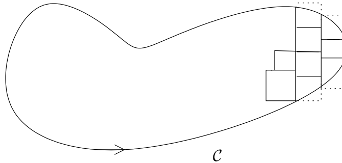
Figure 10: Squares and partial squares
