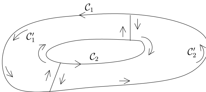
Figure 16: Contours \mathcal{C}_j , \mathcal{C}'_j
